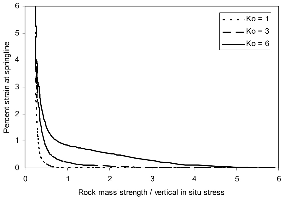
Figure 3. The Effect of shear strength reduction on the developed displacements at the springline
