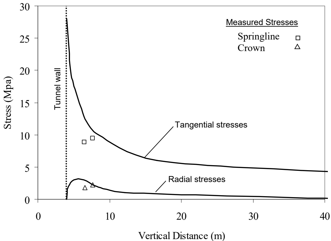
Figure 2. Induced stresses at the tunnel crown due to tunnel excavation
