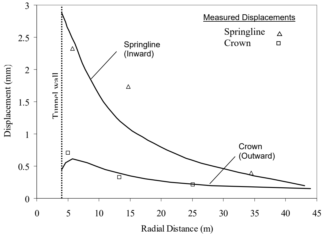
Figure 1. Radial Displacements at the Circumference of Darlington Intake Tunnel
