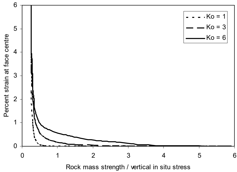
Figure 4. The Effect of shear strength reduction on the developed displacements at the face centre
