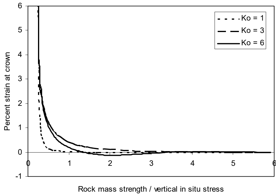
Figure 5. The Effect of shear strength reduction on the developed displacements at the crown
